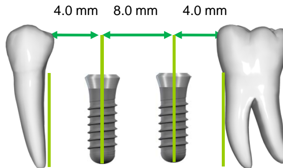
Distance between two RN: tooth/implant, implant/tooth
