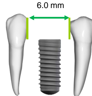
Minimum space for a BL 4.1 mm implant
